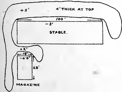
F PLAN OF RETRENCHMENT FOR HORSES AND MAGAZINE IN REAR OF GUN 34 YDS. BACK
